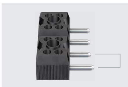
Long version of plug for leading contact
