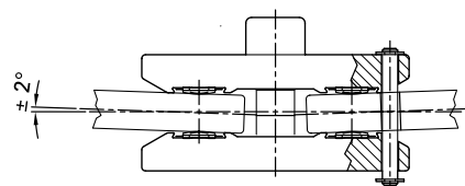
Angular tolerance
